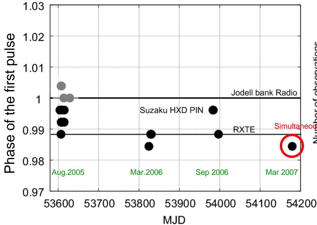
Suzaku HXD PIN, with Jodell bank ephemeris
