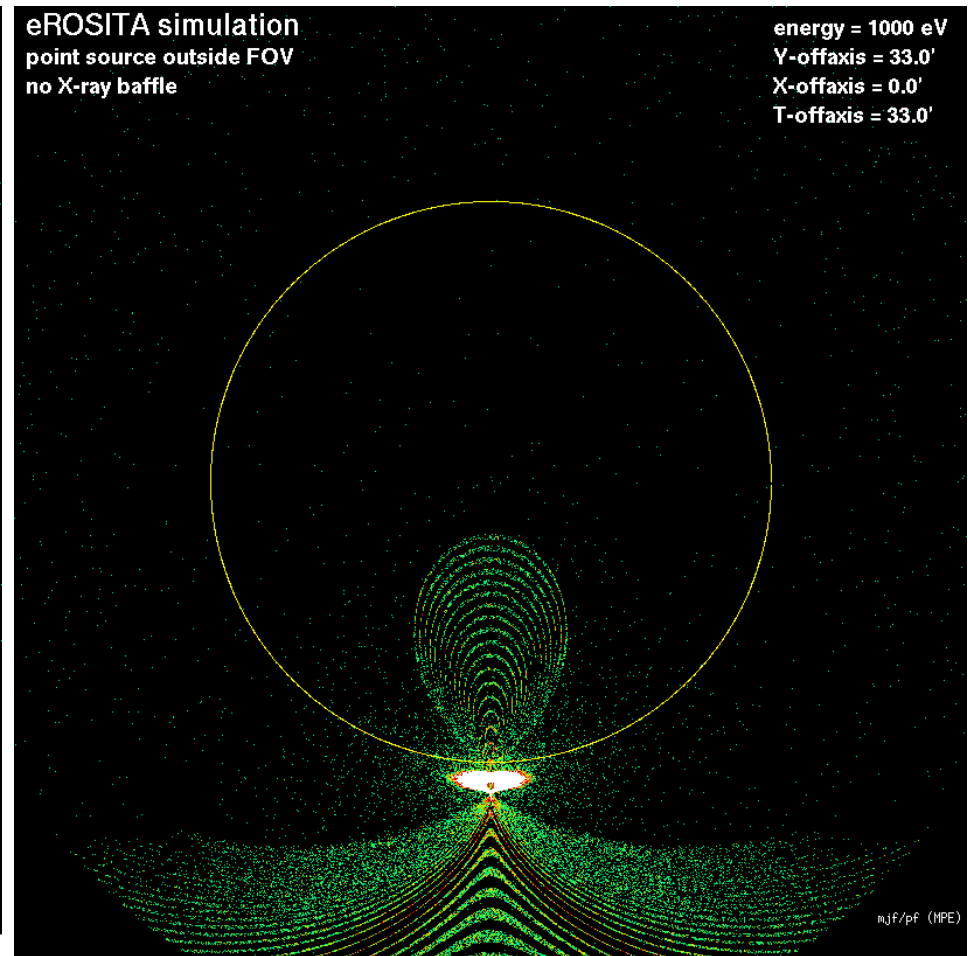
no baffle, no pile-up: bright source off-axis: 32 arcmin (left), 33 arcmin (right)
